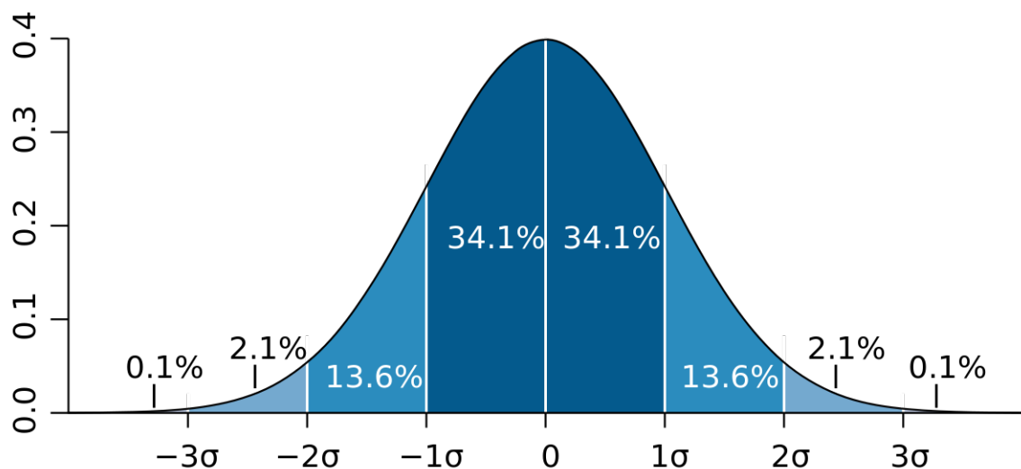
Figure 6.7: Normal Distribution Curve
